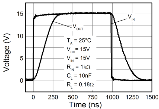
Switching Speed
