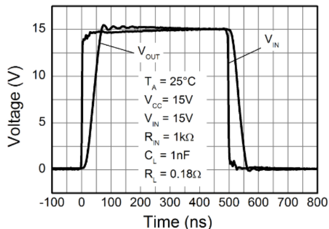
Switching Speed
