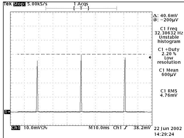
Figure 8. Typical output current waveform under an Over Current Condition. Output current scale at 0.5A/ mV.
