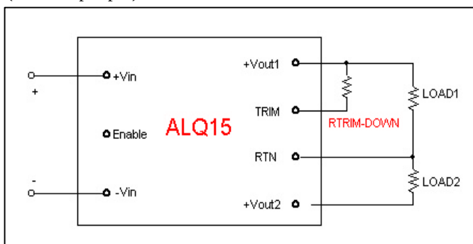
Figure 4. External Trim resistor setup to decrease output for AF; FG; FY and GM standard versions only.
