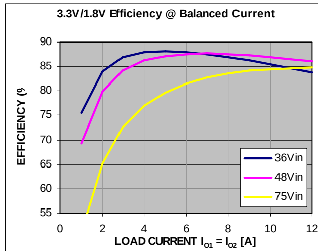
Figure 12. Efficiency curve for balanced output current ( I_{O1} = I_{O2} ) at various input voltages; taken at T_A=25^{\circ}\text{C} with the converter mounted vertically and with 300LFM airflow directed from Pin 3 to Pin 1.
