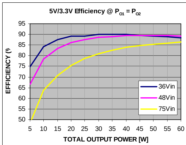
Figure 9. Efficiency at balanced power ( P_{O1} = P_{O2} ) for various input voltages; taken at T_A=25^{\circ}\text{C} with the converter mounted vertically and with 100LFM airflow directed from Pin 3 to Pin 1.
