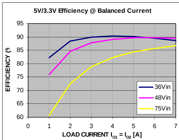
Figure 10. Efficiency curve for balanced output current ( I_{O1} = I_{O2} ) at various input voltages; taken at T_A=25^{\circ}\text{C} with the converter mounted vertically and with 100LFM airflow directed from Pin 3 to Pin 1.
