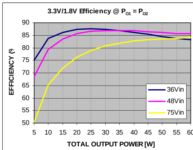
Figure 11. Efficiency at balanced power ( P_{O1} = P_{O2} ) for various input voltages; taken at T_A=25^{\circ}\text{C} with the converter mounted vertically and with 300LFM airflow directed from Pin 3 to Pin 1.
