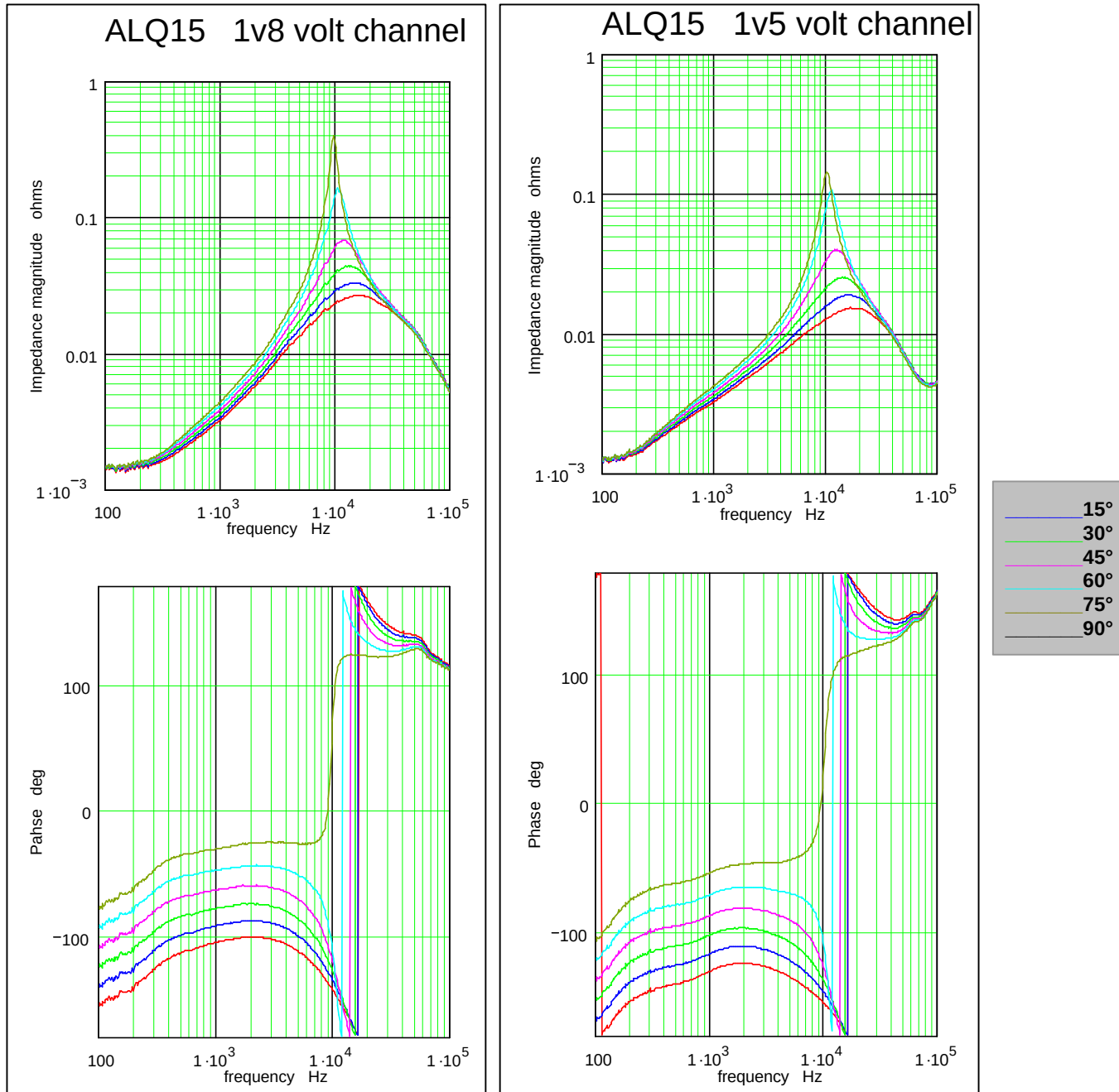
Figure 20. YSC Plots of 1V8 and 1V5 Output Channels.
