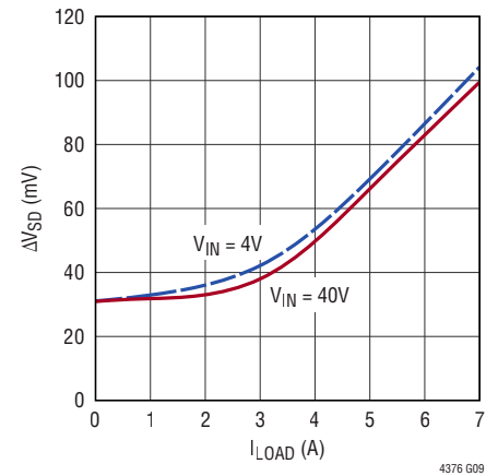
Forward Voltage Drop vs Load Current
