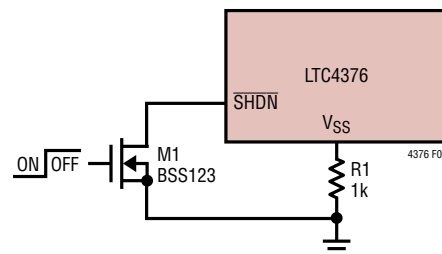
Figure 2. \overline{\text{SHDN}} Control
