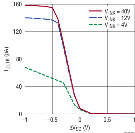
OUTK Current vs Forward Voltage Drop
