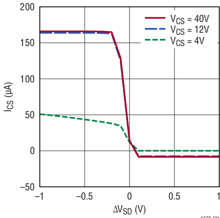
CS Current vs Forward Voltage Drop
