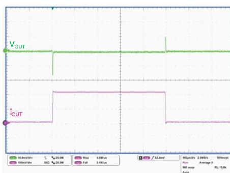
Figure 30: Load transient ( V_{OUT} = V_{ADJ} )
