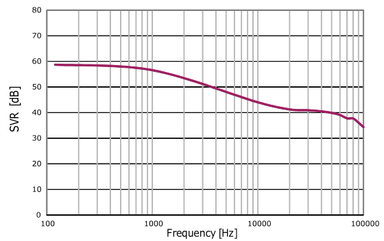
Figure 20: SVR vs. frequency ( V_{OUT} = V_{ADJ} )
