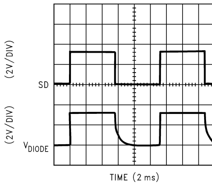
Start-Up Response @ V_{IN} = 3.6V (LM2794)
