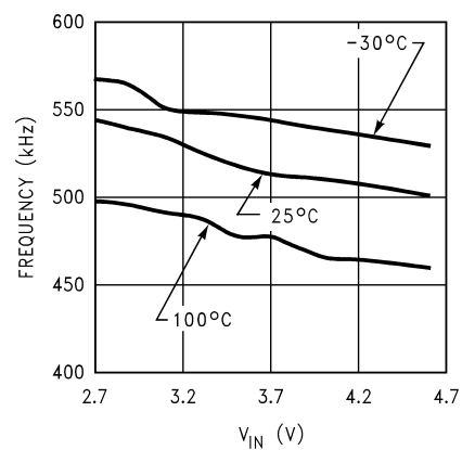
Switching Frequency
