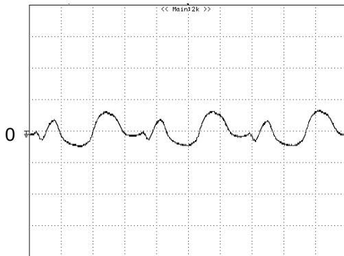
Figure 14: Output voltage ripple at nominal input voltage and rated load current ( I_o=40A ) ( 50\text{ mV/div} , 1\text{ us/div} )
