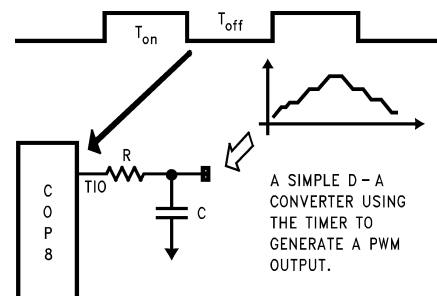
FIGURE 11. Timer Application
