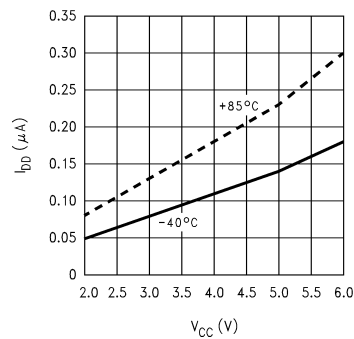
Halt— I_{DD} vs V_{CC} (Brown Out Disabled)
