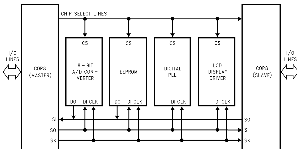
FIGURE 7. MICROWIRE/PLUS Application
