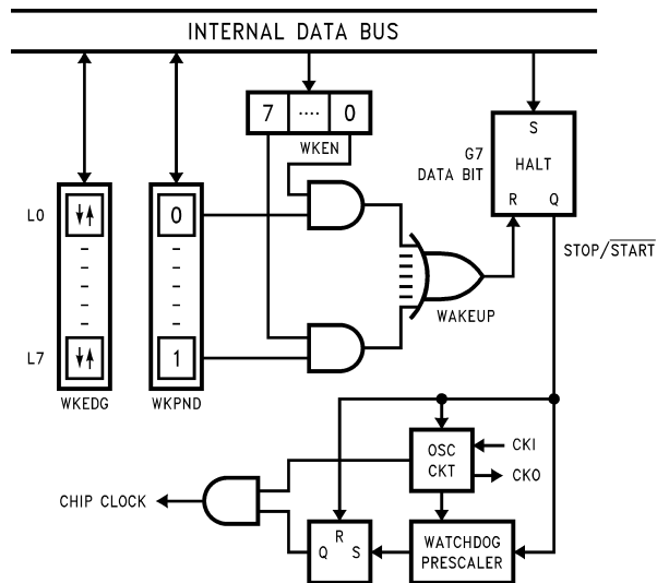
FIGURE 16. Multi-Input Wakeup Logic
