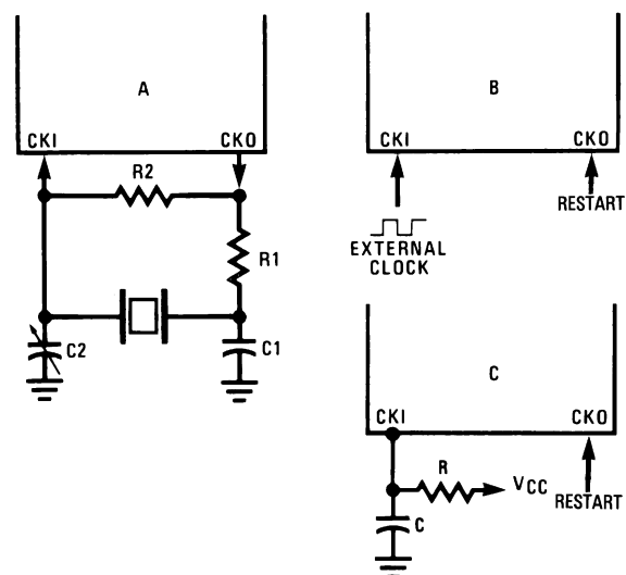
FIGURE 5. Clock Oscillator Configurations
