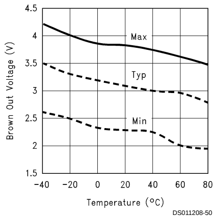
Brown Out Voltage vs Temperature
