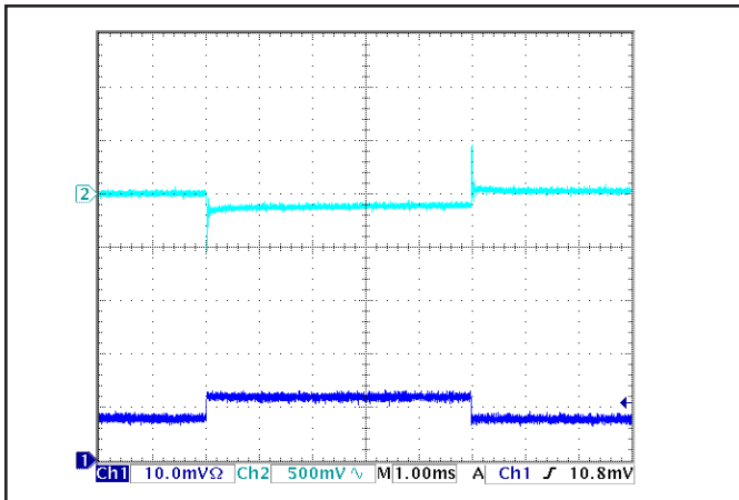
Figure 9: Output voltage response to step-change in load current (50%-75%-50% of I_{out(max)} ; dI/dt = 5A/\mu s ). Load cap: 1uF ceramic and 10uF tantalum capacitors. Top trace: Vout (500mV/div), Bottom trace: Iout (10A/div).
