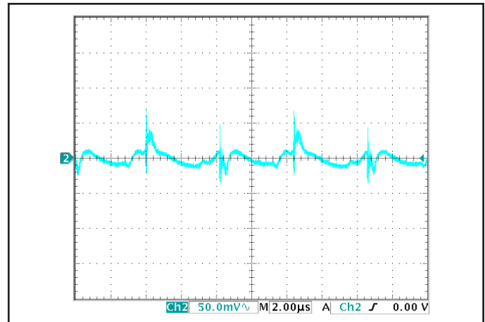
Figure 14: Output voltage ripple at nominal input voltage and rated load current (50mV/div). Load capacitance: 1µF ceramic capacitor and 10µF tantalum capacitor. Bandwidth: 500 MHz. See Figure 11.
