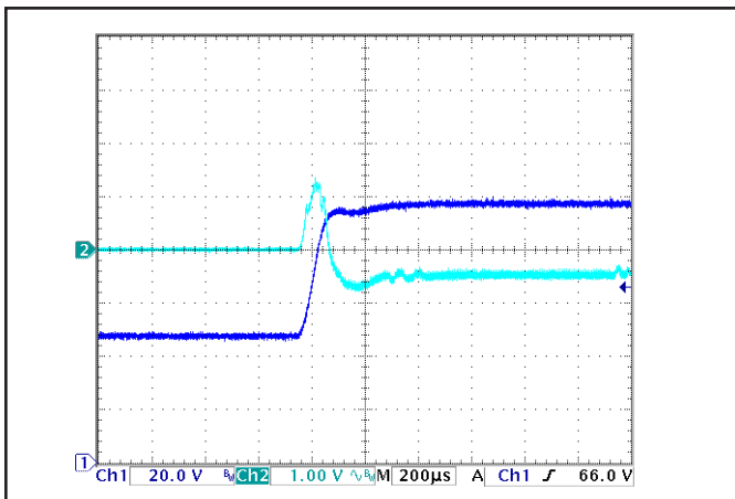
Figure 15: Output voltage response to step-change in input voltage (50V to 100V in 200µs). Load cap: 470µF, 15 mΩ ESR tantalum capacitor. Ch 1: V_{in} (20V/div), Ch 2: V_{out} (1V/div), at zero load current.
