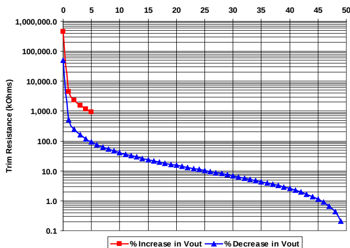
Figure B: Trim Graph for 12Vout module
