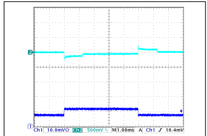
Figure 10: Output voltage response to step-change in load current (50%-75%-50% of I_{out(max)} ; dI/dt = 5A/\mu s ). Load cap: 470μF, 15 mΩ ESR tantalum capacitor. Top trace: Vout (500mV/div), Bottom trace: Iout (10A/div).
