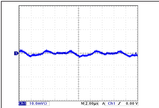
Figure 13: Input reflected ripple current, i_s , through a 4.7µH source inductor, using a 100µF input capacitor, at nominal input voltage and rated load current (10mA/div). See Figure 11.
