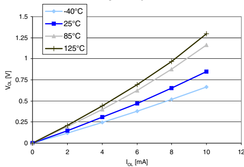
Figure 27. Typ. V_{OL} @ V_{DD} = 5.0 V (standard ports)
