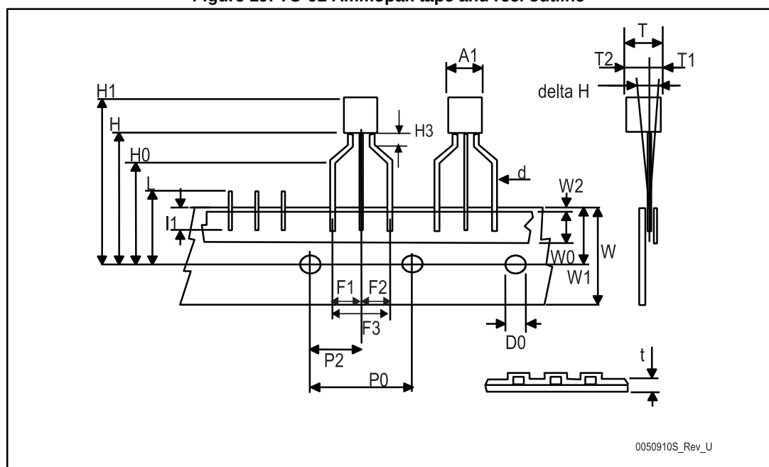
Figure 19: TO-92 Ammopak tape and reel outline
