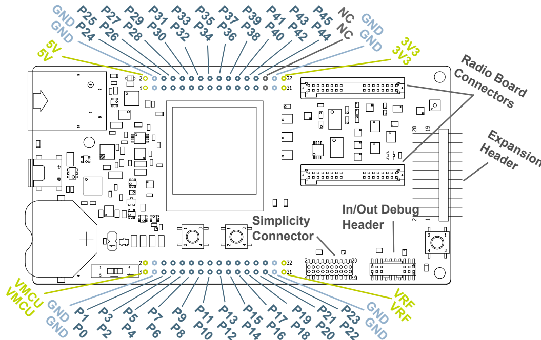
Figure 4.1 Connector Layout
