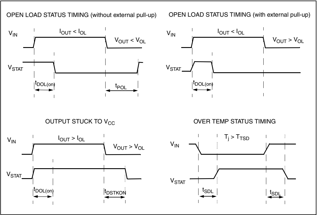
Figure 4. Status timings
