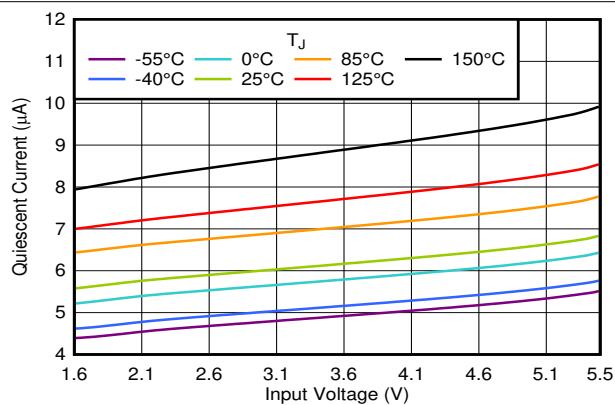
Figure 6-36. I_{GND} vs V_{IN} in the Dropout Region
