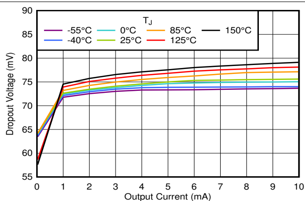
Figure 6-26. Dropout Voltage vs I_{OUT}
