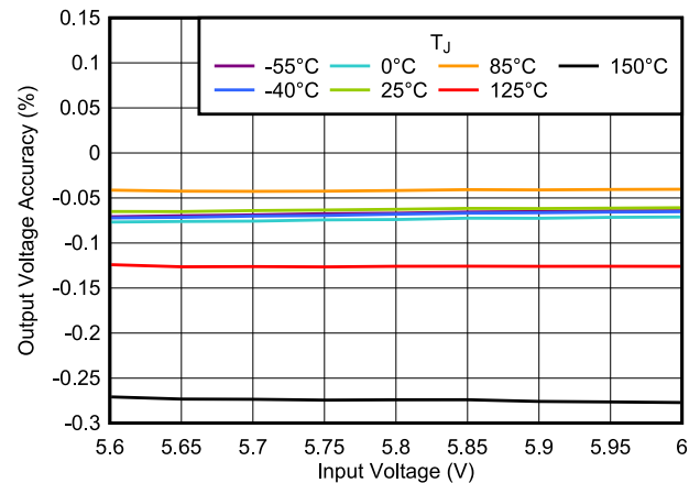
Figure 6-22. Output Voltage Accuracy vs V_{IN}
