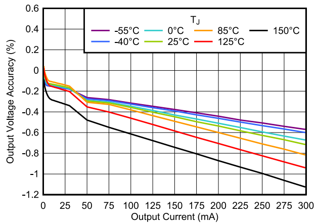
Figure 6-13. Output Voltage Accuracy vs I_{OUT}
