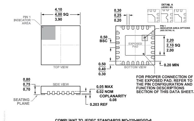
Figure 37. 24-Lead Lead Frame Chip Scale Package (LFCSP) 4 mm x 4 mm Body and 0.75 mm Package Height (CP-24-10) Dimension shown in millimeters
