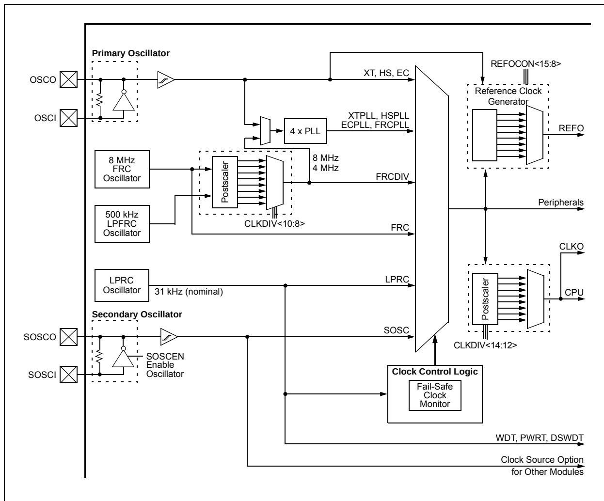
FIGURE 9-1: PIC24EXXXXXX FAMILY CLOCK DIAGRAM
