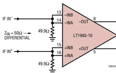
Figure 2. Input Termination for Differential 50 \Omega Input Impedance
