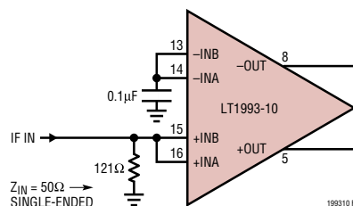
Figure 1. Input Termination for Single-Ended 50 \Omega Input Impedance
