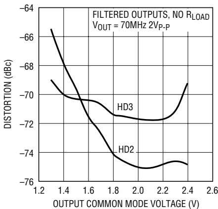
Distortion vs Output Common Mode Voltage, LT1993-10 Driving LTC2249 14-Bit ADC
