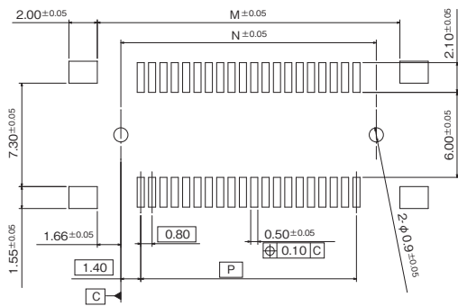
Recommended P.C.B. layout (View from mounting side)
