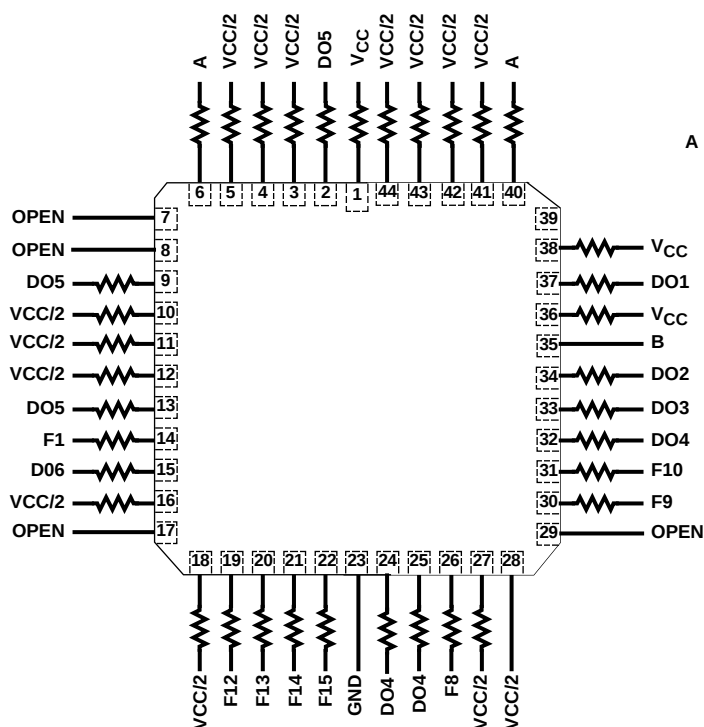
MR82C37A CLCC
