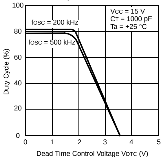
Fig. 31 -Duty Cycle vs. Dead Time Control Voltage
