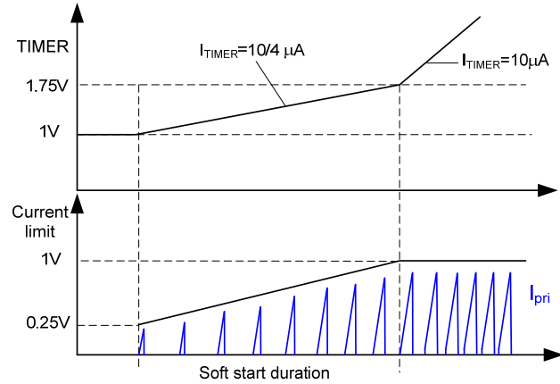
Figure 6: Soft-Start
