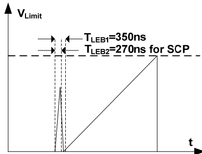
Figure 10: Leading-Edge Blanking
