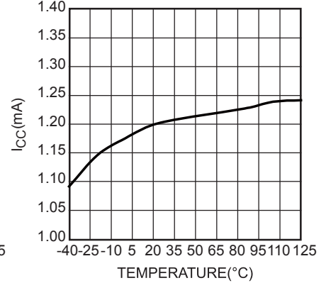
Internal IC Consumption vs. Temperature
