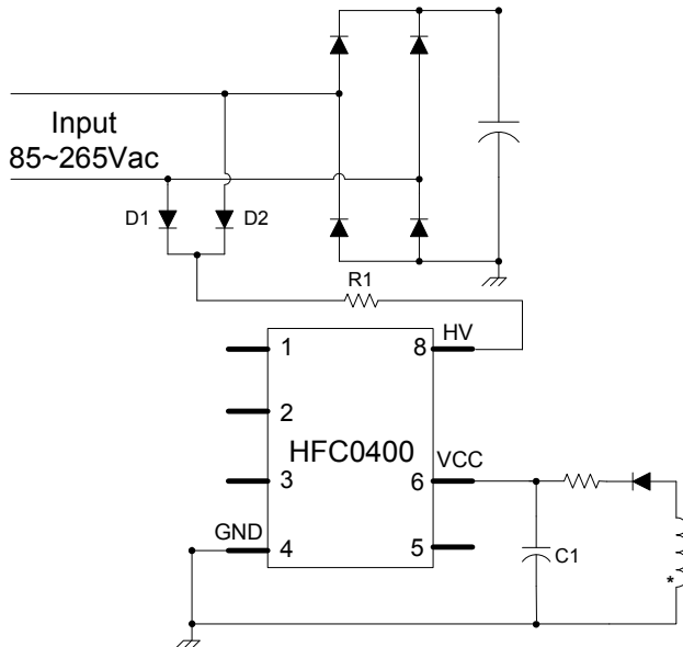
Figure 11: Start-Up Circuit
