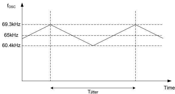
Figure 3: Frequency Jitter
