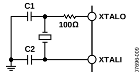
Figure 9. Crystal Oscillator Circuit
