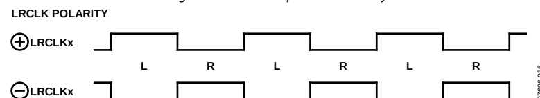
Figure 35. Serial Output LRCLK Polarity
