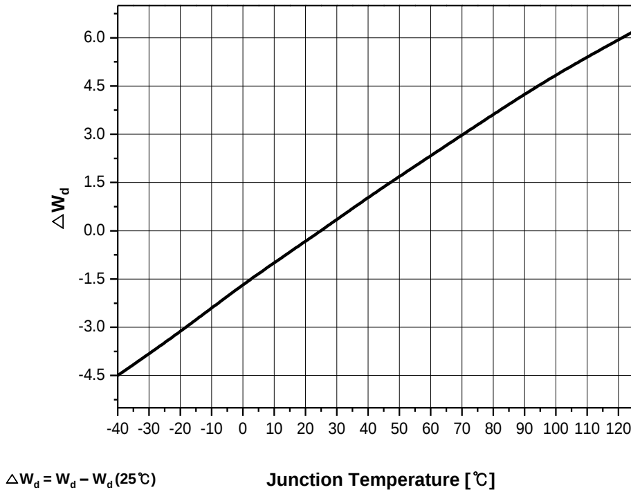
Fig 8. Dominant wavelength shift vs. Junction Temperature, I_F = 20\text{mA}
