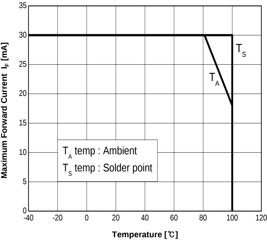
Fig 9. Maximum Forward Current vs. Temperature
