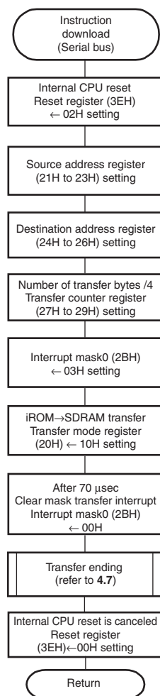
(a) Transfer over 1 Kbytes
