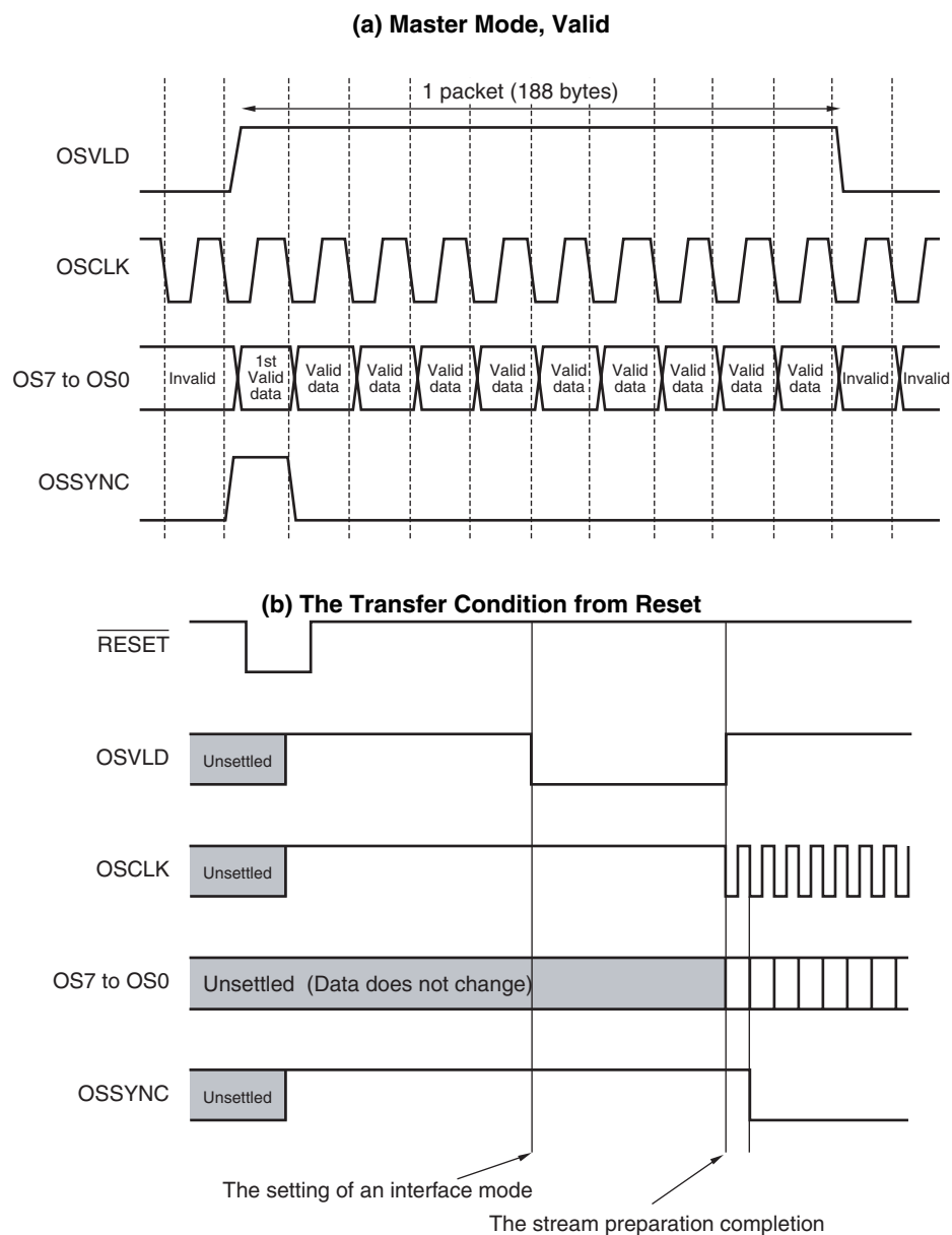
Figure 2-8. Parallel Stream Transmission Mode ; Transmission of MPEG2-TS (Packet Length is 188 Bytes)
