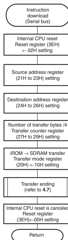
(b) Transfer below 128 bytes
