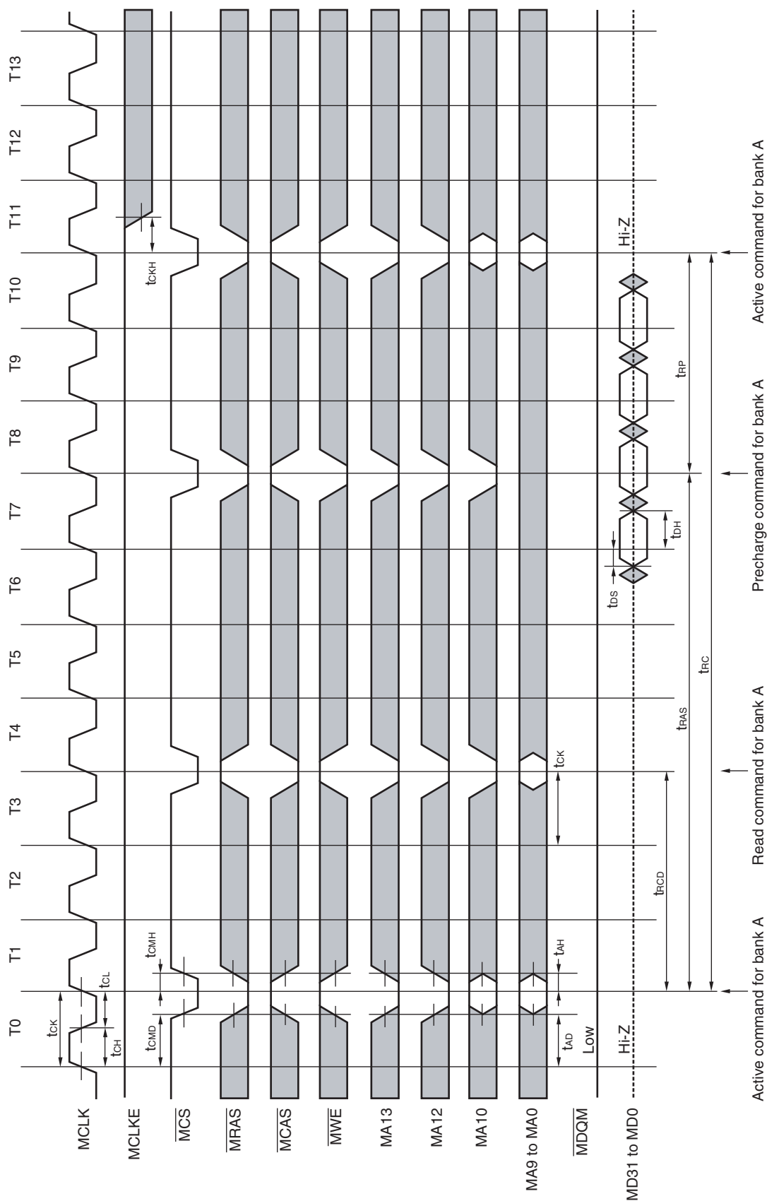
Read timing (Manual pre-charge, burst length = 4, CAS latency = 3)
