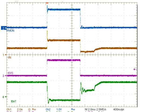
Figure 32. Transient Response, Charge Disabled, In Supplement Mode
