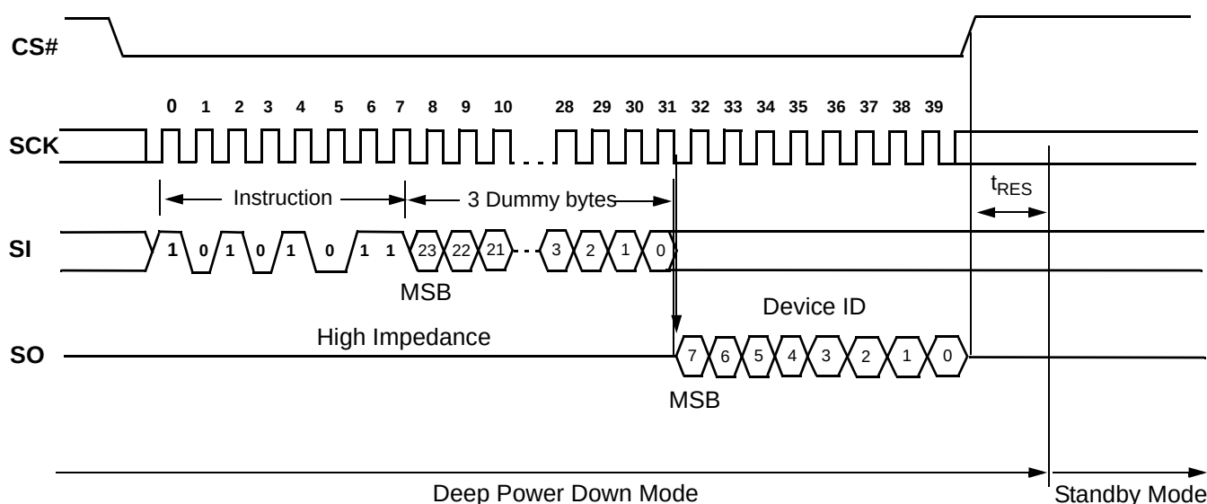
Figure 18. Release from Deep Power Down and Read Electronic Signature (RES) Instruction Sequence
