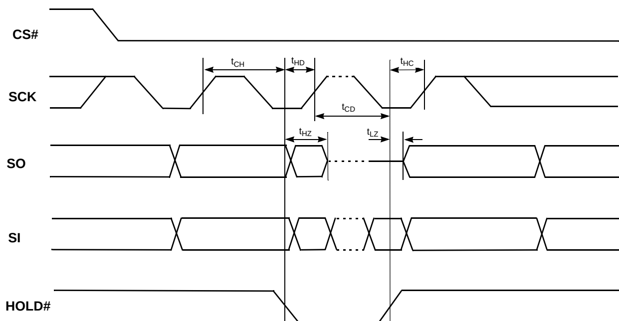
Figure 27. HOLD# Timing
