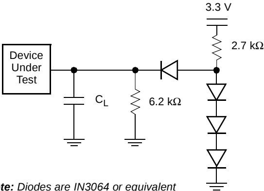
Figure 11. Test Setup
