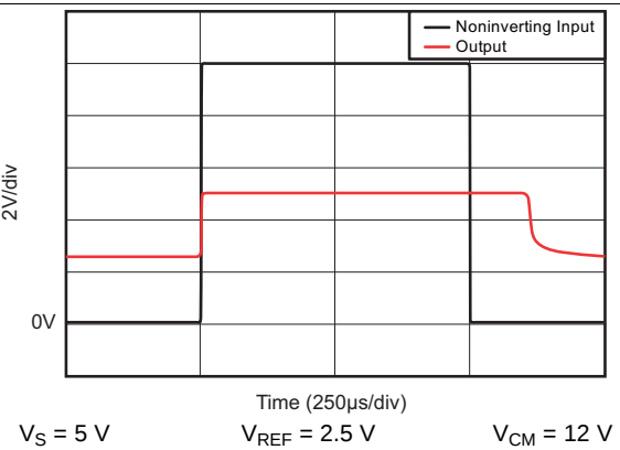
图 20. Noninverting Differential Input Overload
