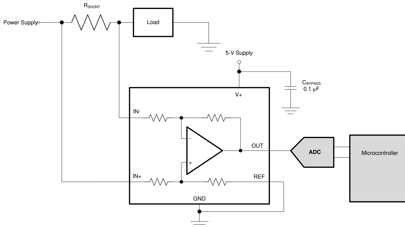
图 23. Typical Application
