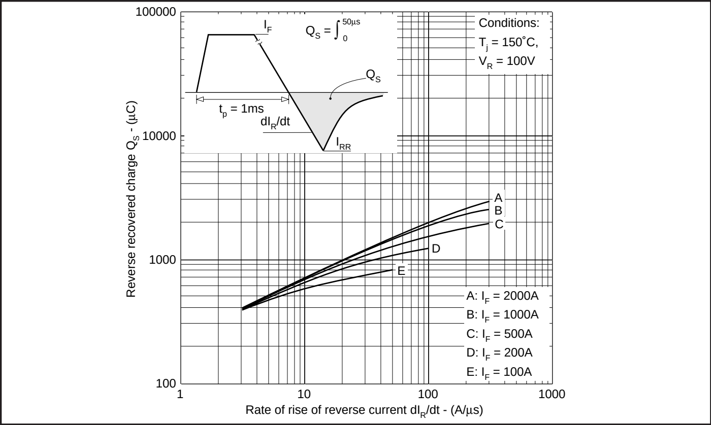
Fig.3 Recovered charge
