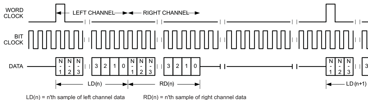
Figure 5-26. Timing Diagram for DSP Mode
