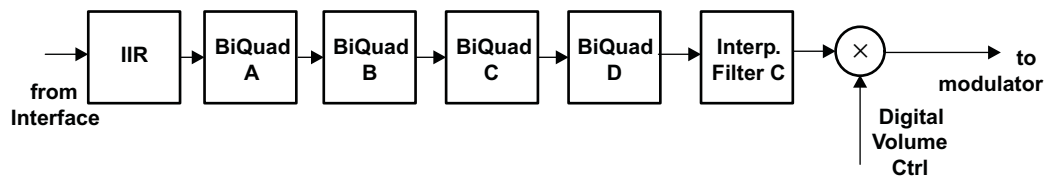
Figure 5-9. Signal Chain for PRB_P22
