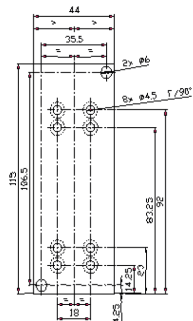
MPA 500 thickness = 5mm
