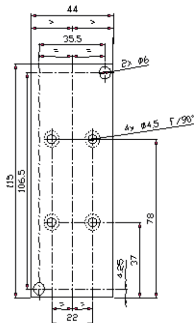
MPA 250 thickness = 2.5mm
