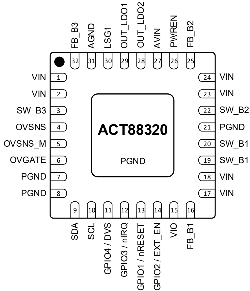
Figure 1: Pin Configuration – Top View – QFN44-32
