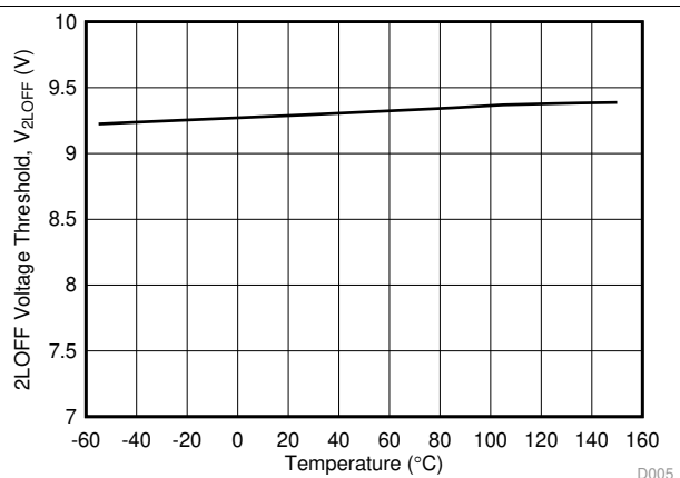
Figure 27. V_{2LOFF} 2-Level Turn Off Voltage Threshold vs. Temperature
