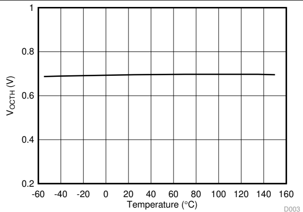
Figure 25. V_{OCTH} OC Detection Threshold vs. Temperature
