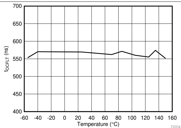
Figure 26. t_{OFLT} OC to \overline{FLT} Low Delay Time vs. Temperature
