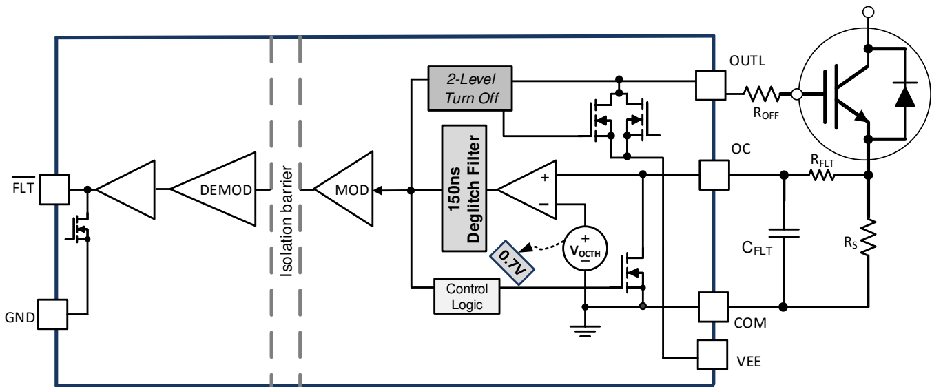
Figure 44. 2-Level Turn-off
