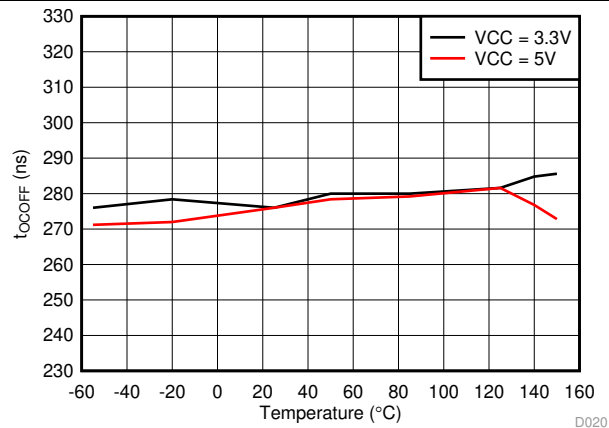
Figure 24. t_{OCOFF} OC Propagation Delay vs. Temperature
