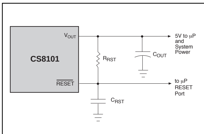
Figure 3. RC Network for \overline{\text{RESET}} Delay
