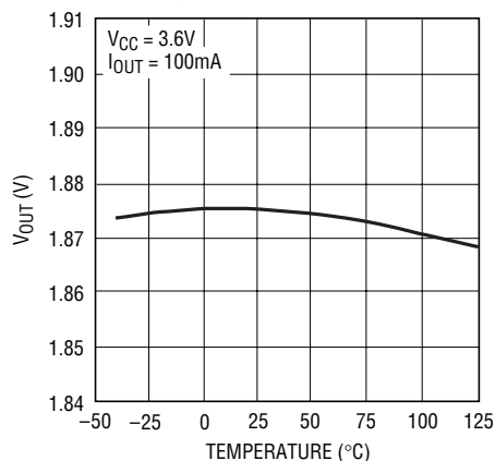
Buck Regulator Output Voltage vs Temperature
