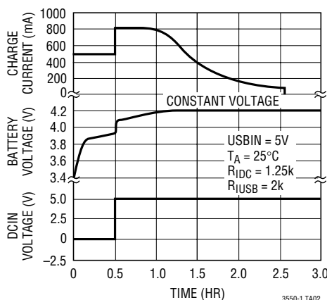
Complete Charge Cycle (1100mA Battery)
