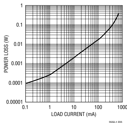
Figure 3. Power Lost vs Load Current
