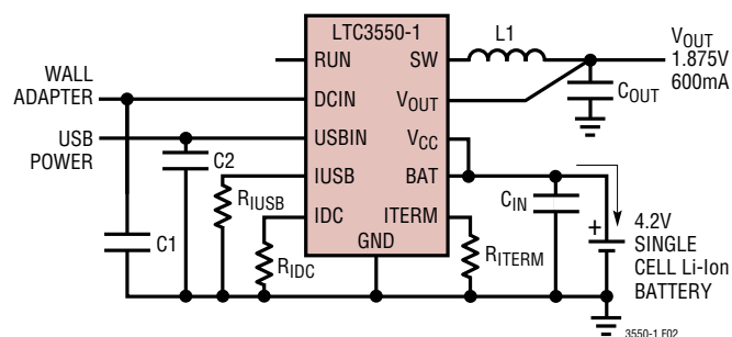
Figure 2. LTC3550-1 Basic Circuit
