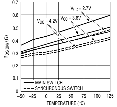
Buck Regulator Switches R_{DS(ON)} vs Temperature
