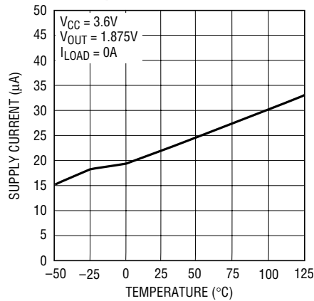
Buck Regulator Supply Current vs Temperature
