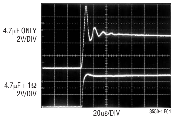
Figure 4. Waveforms Resulting from Hot-Plugging a 5V Input Supply When Using Ceramic Bypass Capacitors
