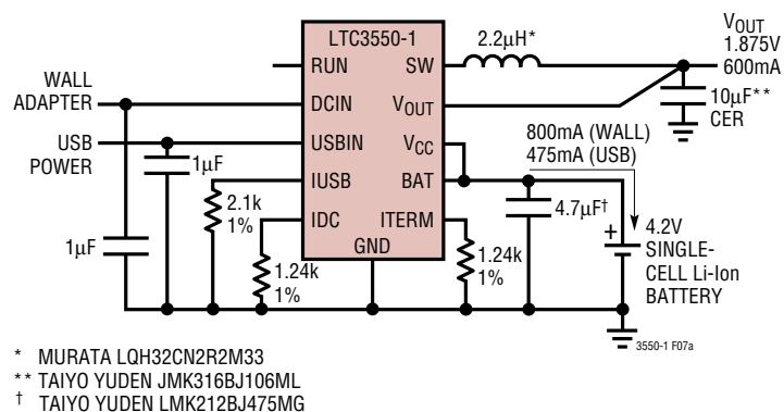
Figure 7a. Design Example Circuit
