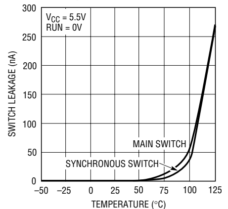
Switch Leakage Current vs Temperature
