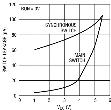
Switch Leakage Current vs V_{CC}
