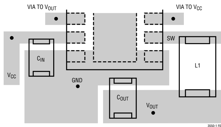
Figure 6. DC-DC Converter Suggested Layout
