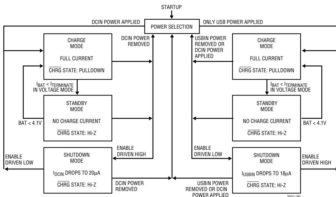
Figure 1. LTC3550-1 State Diagram of a Charge Cycle
