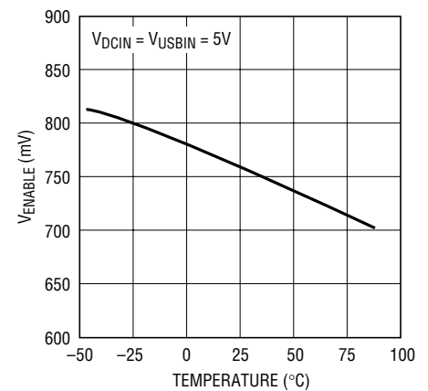
ENABLE Pin Threshold Voltage (On-to-Off) vs Temperature
