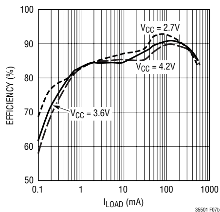
Figure 7b. Buck Regulator Efficiency vs Output Current
