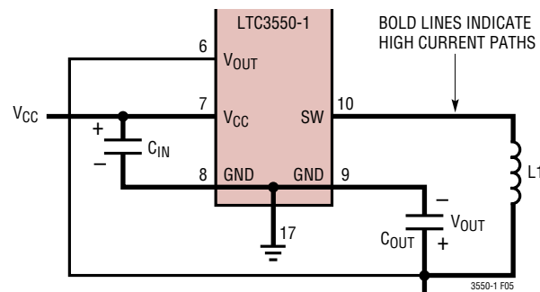
Figure 5. DC-DC Converter Layout Diagram
