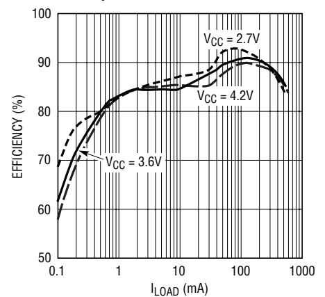
Buck Regulator Efficiency vs Output Current
