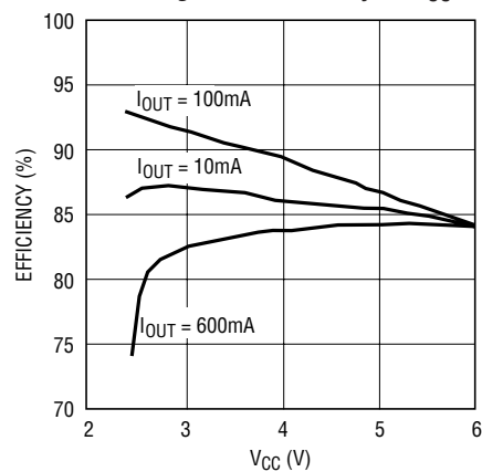
Buck Regulator Efficiency vs V_{CC}
