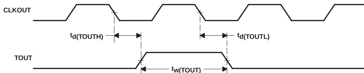
Figure 5–19. TOUT Timing
