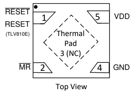
DPW Package (Preview) 5-Pin X2SON Top View
