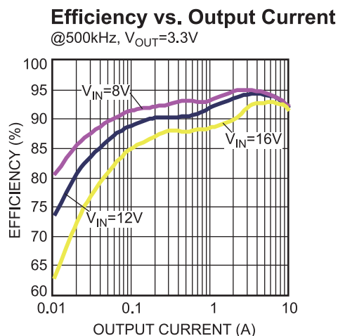
Figure 46 — Efficiency Curve
