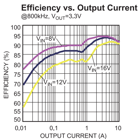
Figure 48 — Efficiency Curve
