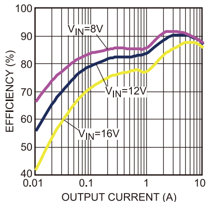
Figure 34 — Efficiency Curve
