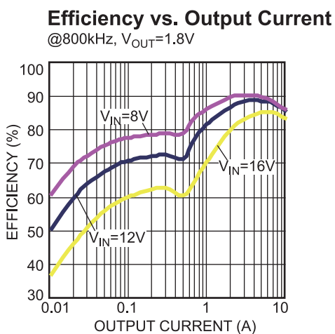
Figure 42 — Efficiency Curve
