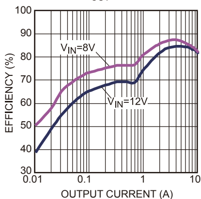
Figure 20 — Efficiency Curve
