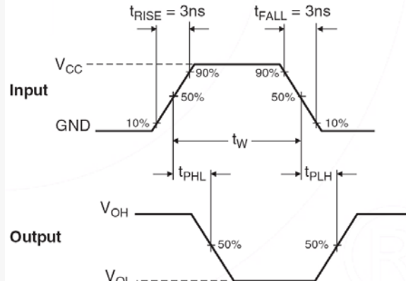
Figure 5. AC Waveforms
