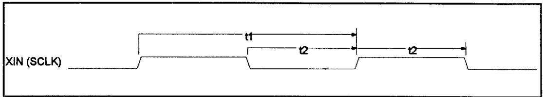
FIGURE 29 - CLOCK TIMING
