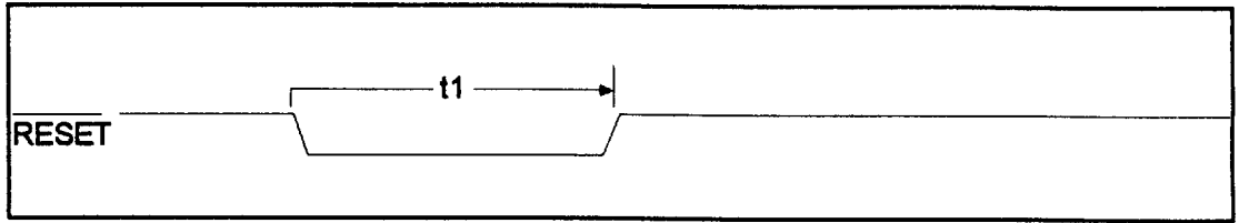
FIGURE 28 - RESET TIMING
