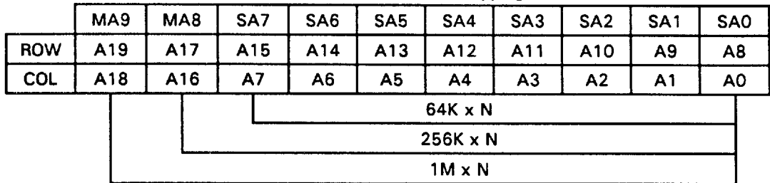
DRAM Linear Address Mapping
