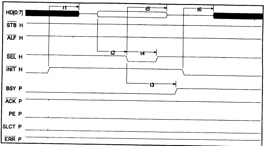
FIGURE 11 - SPP ADDRESS WRITE TIMING (PARALLEL PORT SIGNALS)
