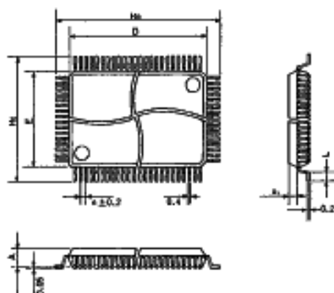
QFP/QFPS
