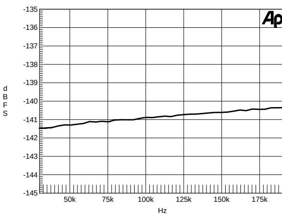
Figure 42. Dynamic Range vs. Output Sample Rate, -60 dBFS 1 kHz Tone, Fsi = 192 kHz
