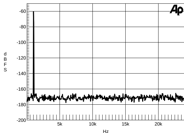
Figure 23. Wideband FFT Plot (16k Points) -60 dBFS 1 kHz Tone, 48 kHz:48 kHz
