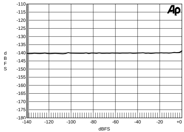
Figure 58. THD+N vs. Input Amplitude, 1 kHz Tone, 48 kHz:96 kHz
