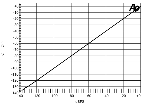
Figure 56. Linearity Error, 0 to -140 dBFS Input, 200 Hz Tone, 192 kHz:44.1 kHz
