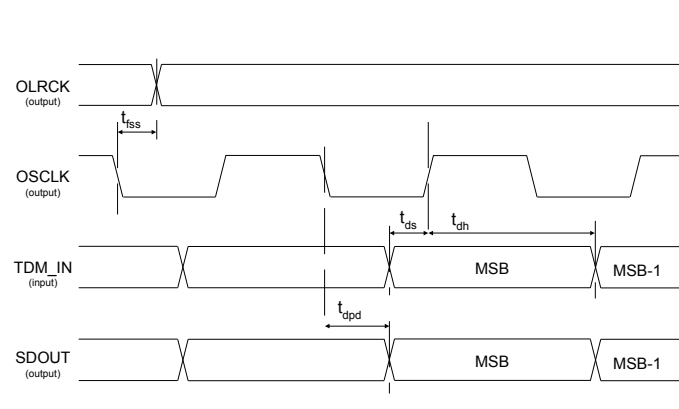
Figure 4. TDM Master Mode Timing
