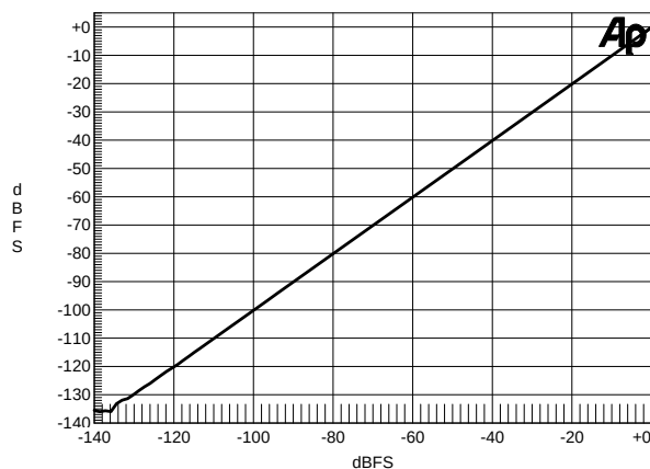
Figure 55. Linearity Error, 0 to -140 dBFS Input, 200 Hz Tone, 44.1 kHz:48 kHz
