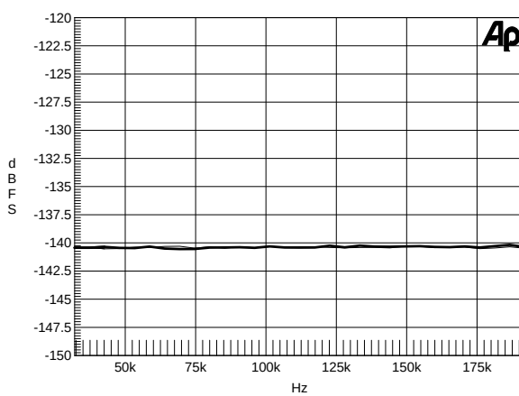
Figure 44. Dynamic Range vs. Output Sample Rate, -60 dBFS 1 kHz Tone, Fsi = 32 kHz
