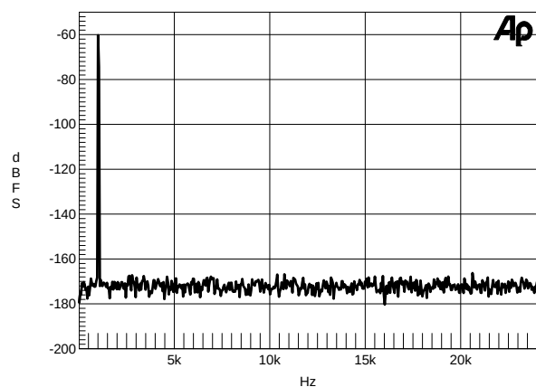
Figure 27. Wideband FFT Plot (16k Points) -60 dBFS 1 kHz Tone, 96 kHz:48 kHz
