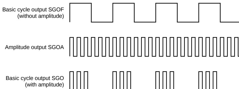
Figure 18-2: Concept of Each Signal
