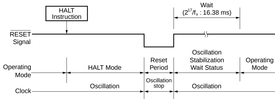
Figure 21-4: HALT Mode Release by \overline{\text{RESET}} Input
