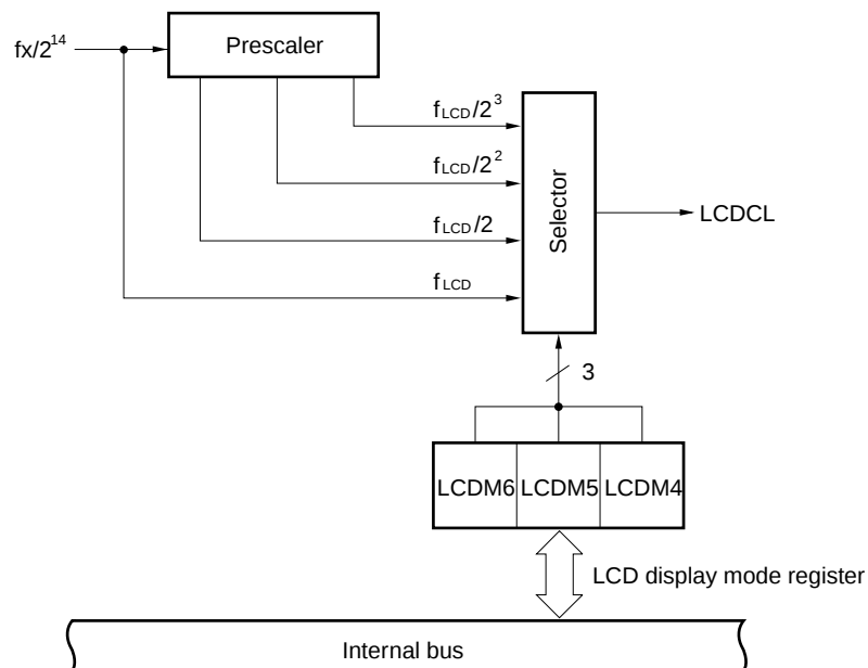
Figure 17-2: LCD Clock Select Circuit Block Diagram
