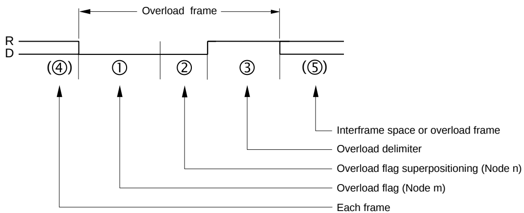
Figure 16-15: Overload Frame
