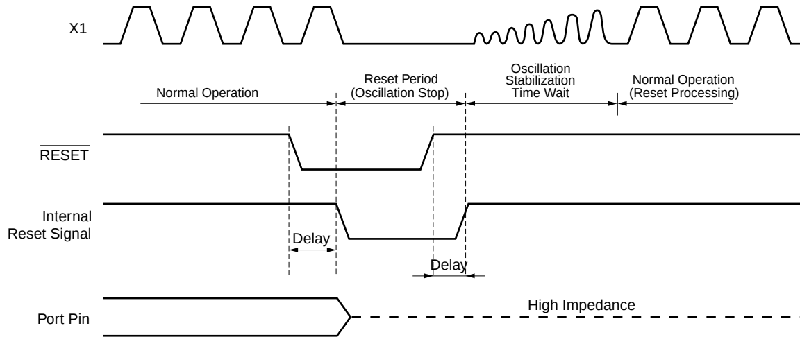
Figure 22-2: Timing of Reset Input by \overline{\text{RESET}} Input
