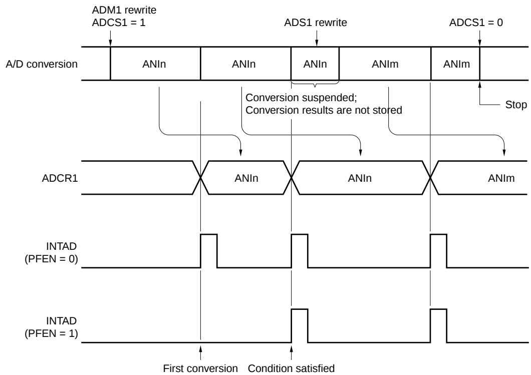
Figure 12-9: A/D Conversion
