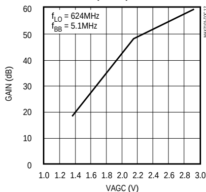
RF SIGNAL PATH GAIN vs. AGC (PIN 93) VOLTAGE
