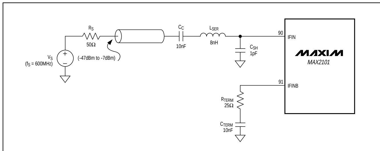
Figure 14. Example of Input Network to Minimize VSWR and Noise Figure
