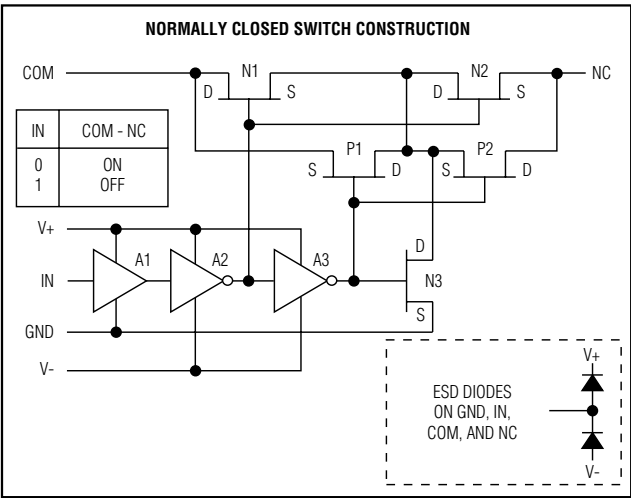
Figure 1. T-Switch Construction
