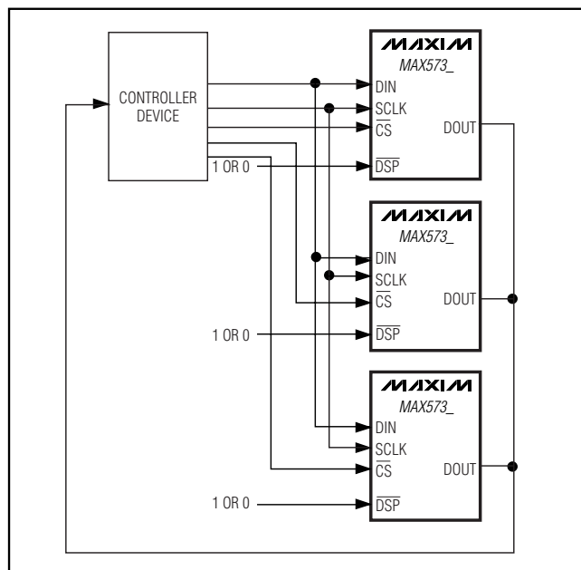
Figure 8. Example of a Parallel Configuration with Read-Back
