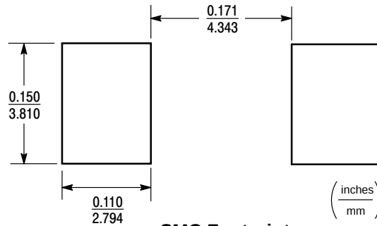
SMC Footprint
