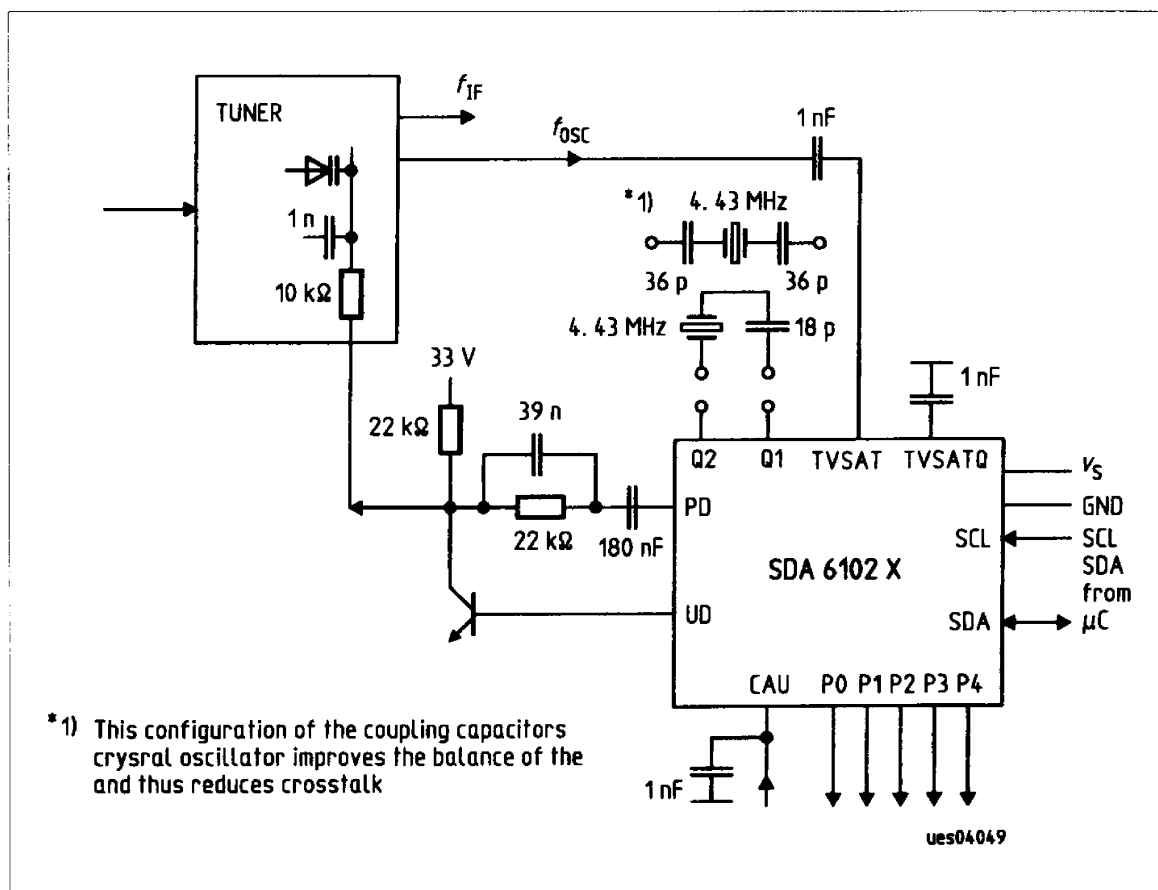
Application Circuit
