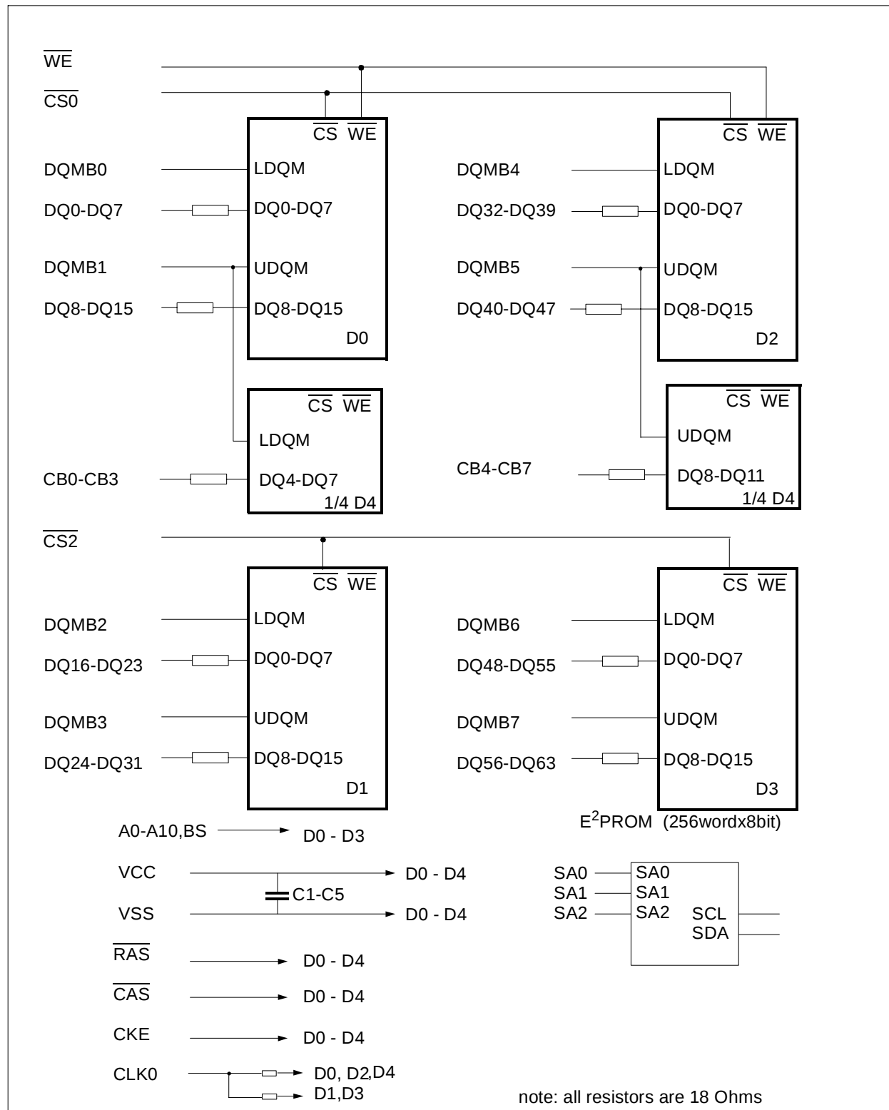
Block Diagram for 1M x 72 SDRAM - DIMM module
