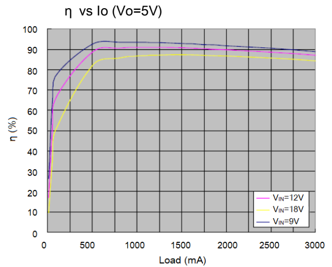
Figure 2. Typical Efficiency Curve
