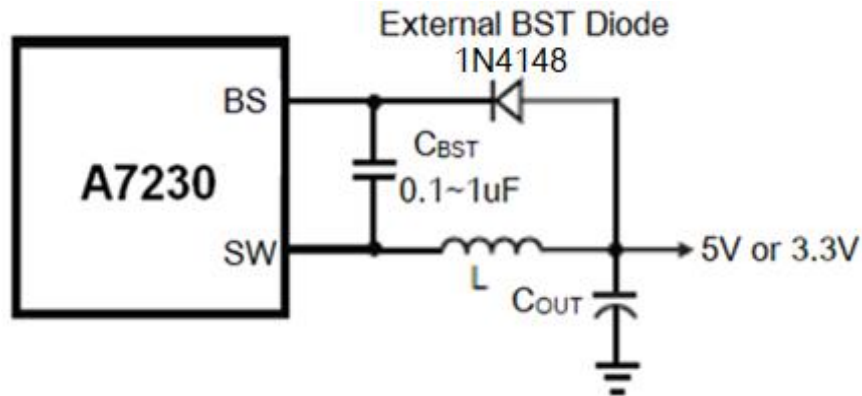
Add Optional External Bootstrap Diode to Enhance Efficiency
