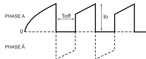
Fig.1 Constant current wave form (Motor current)
